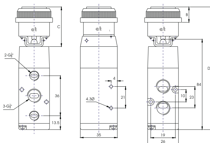
MSV-86521- 3/2 Mechanical Valve
