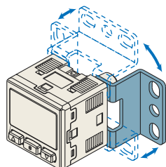
Bracket B/C
